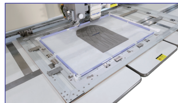
工装夹具 Specialized Fixtures
