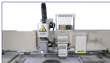
任意转缝绉机头+精密绣花机头 Freely rotating sewing head + precision embroidery head
